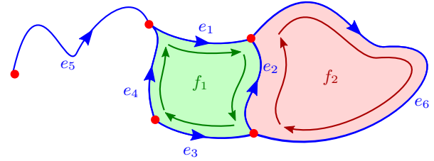
Figure 6: Two faces f_1 and f_2 each defined by one cycle. The cycle defining f_1 is [(e_1, \text{true}); (e_2, \text{false}); (e_3, \text{false}); (e_4, \text{true})] , while the cycle defining f_2 is [(e_2, \text{true}); (e_6, \text{true})] .
