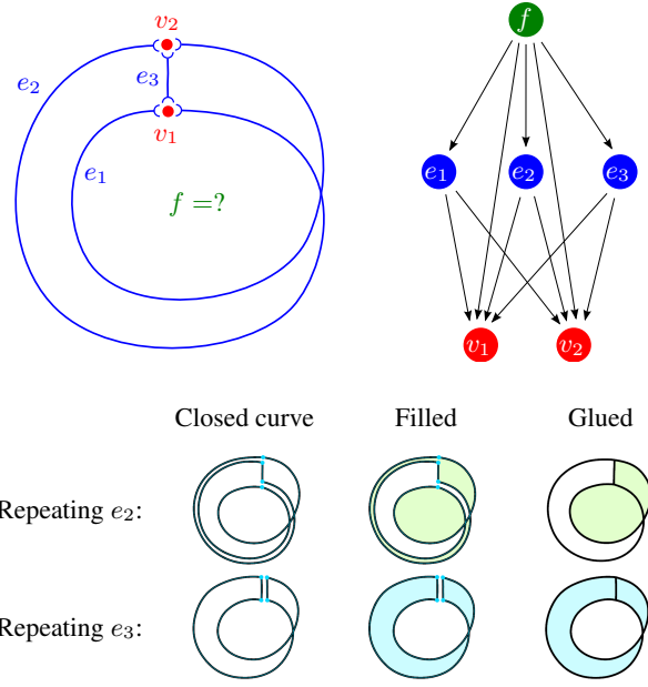
Figure 9: Top: The incidence graph (without semantics) of a Möbius strip. Bottom: To render it, one needs to decompose its boundary into a closed curve. This requires to repeat (at least) one edge, and this choice is ambiguous: repeating e_2 or repeating e_3 give different rendering results when filling the face using the even-odd winding rule.
