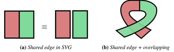
Figure 3: The limitations of existing representations. SVG cannot represent two faces sharing a common edge as in (a), therefore must duplicate the shared edge. Planar maps can represent shared edges, but cannot represent overlapping faces, thus neither SVG nor planar maps can represent the illustration in (b).
